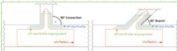
SAERTEX® multiHat combi Adjustment 90° Connection
